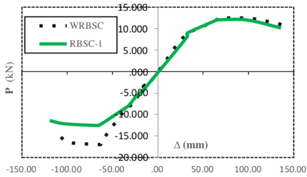
Fig. 5. The relation between load and displacement.
