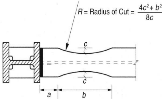
Fig. 1. RBS design on beam flange.
