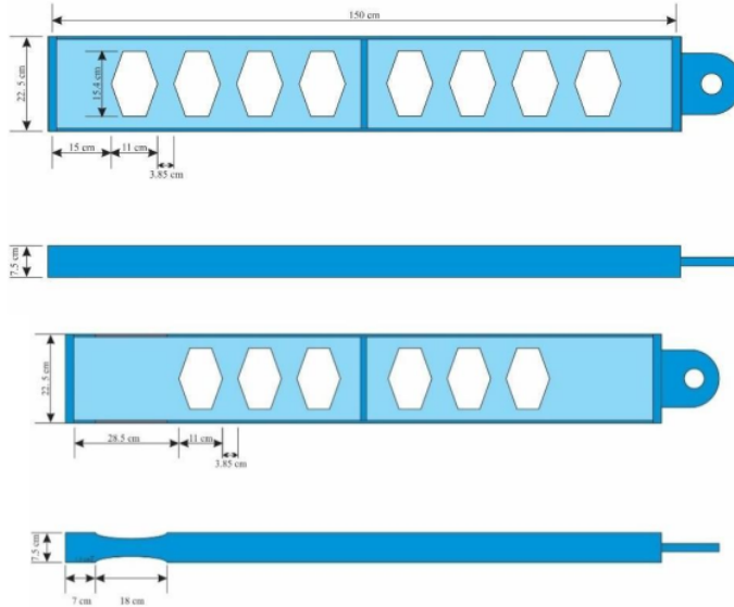
Fig. 2. The dimension of castellated beam and RBS.
